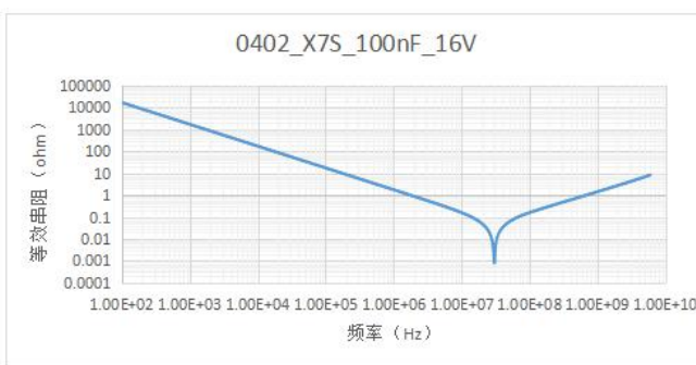
Equivalent series resistance (ESR) characteristic curve
